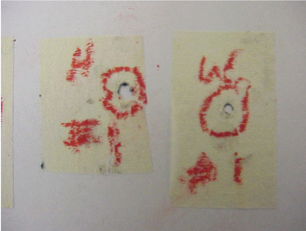
Helmet Photograph 21. Penetration Failure - AFX, FX-28, S (56-57 cm)
