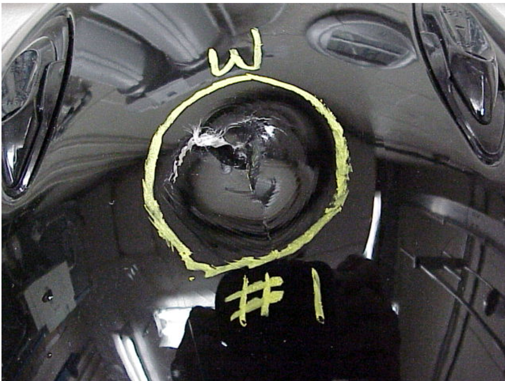
Helmet Photograph 18. Penetration Failure – Water Immersed AFX, FX-28, S (56-57 cm)
