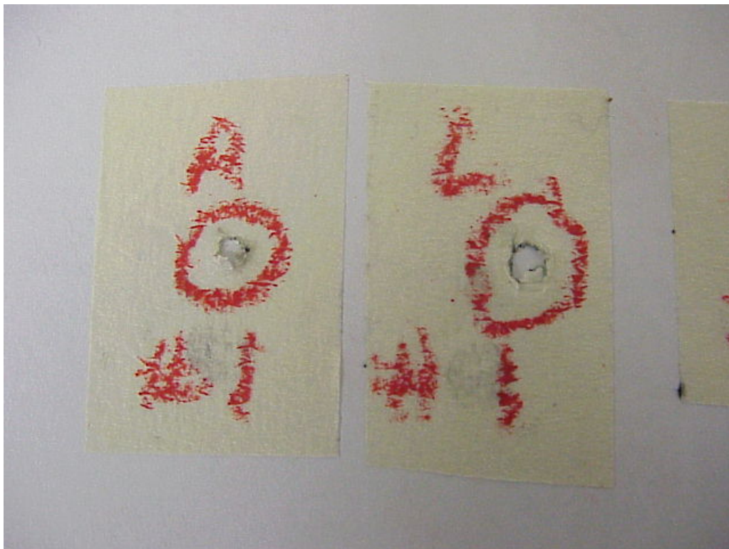
Helmet Photograph 20. Penetration Failure - AFX, FX-28, S (56-57 cm)
